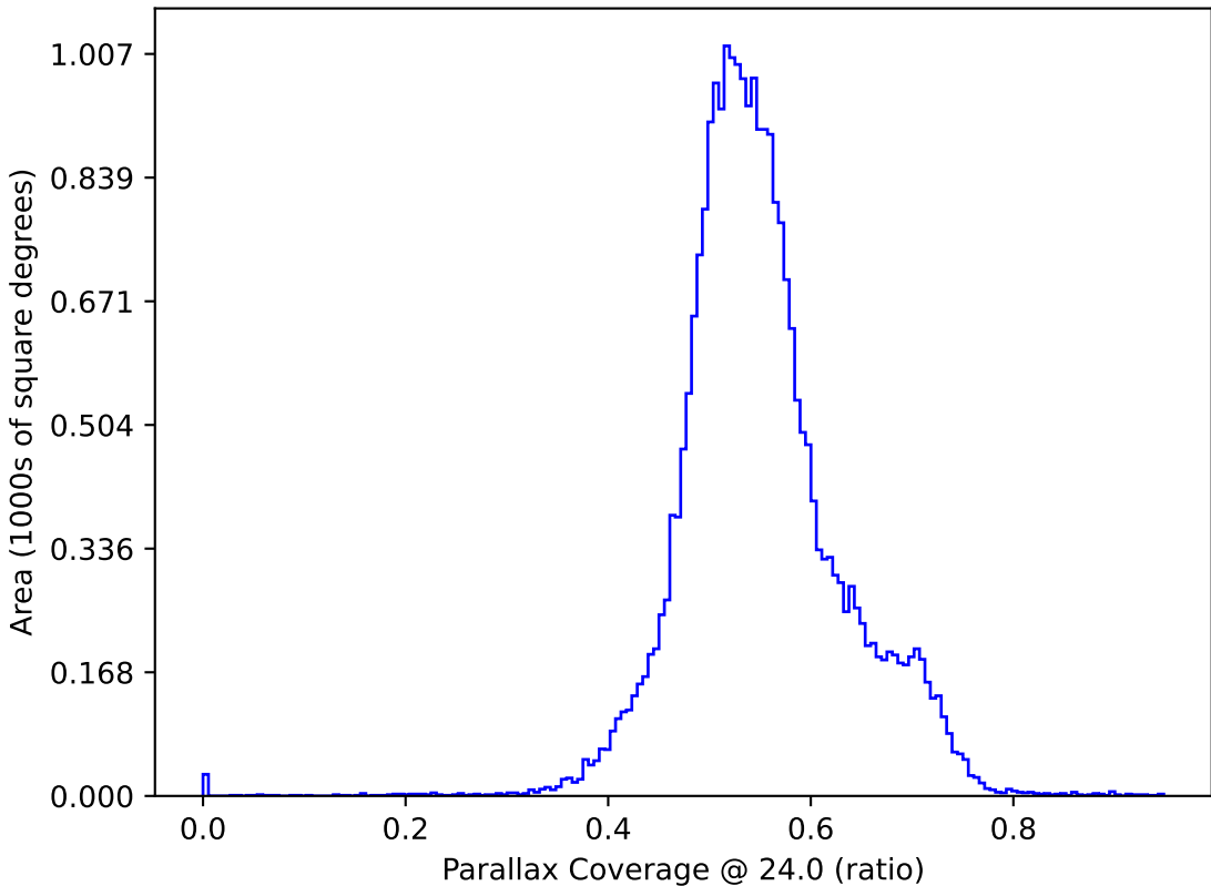
too_elab_r32_d3_gz_v3.4_10yrs : Parallax Coverage @ 24.0
