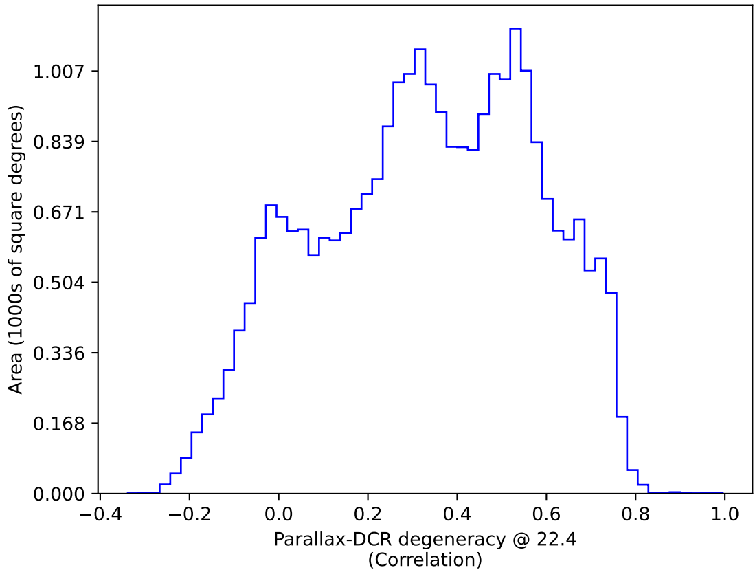
too_elab_r32_d3_gz_v3.4_10yrs : Parallax-DCR degeneracy @ 22.4
