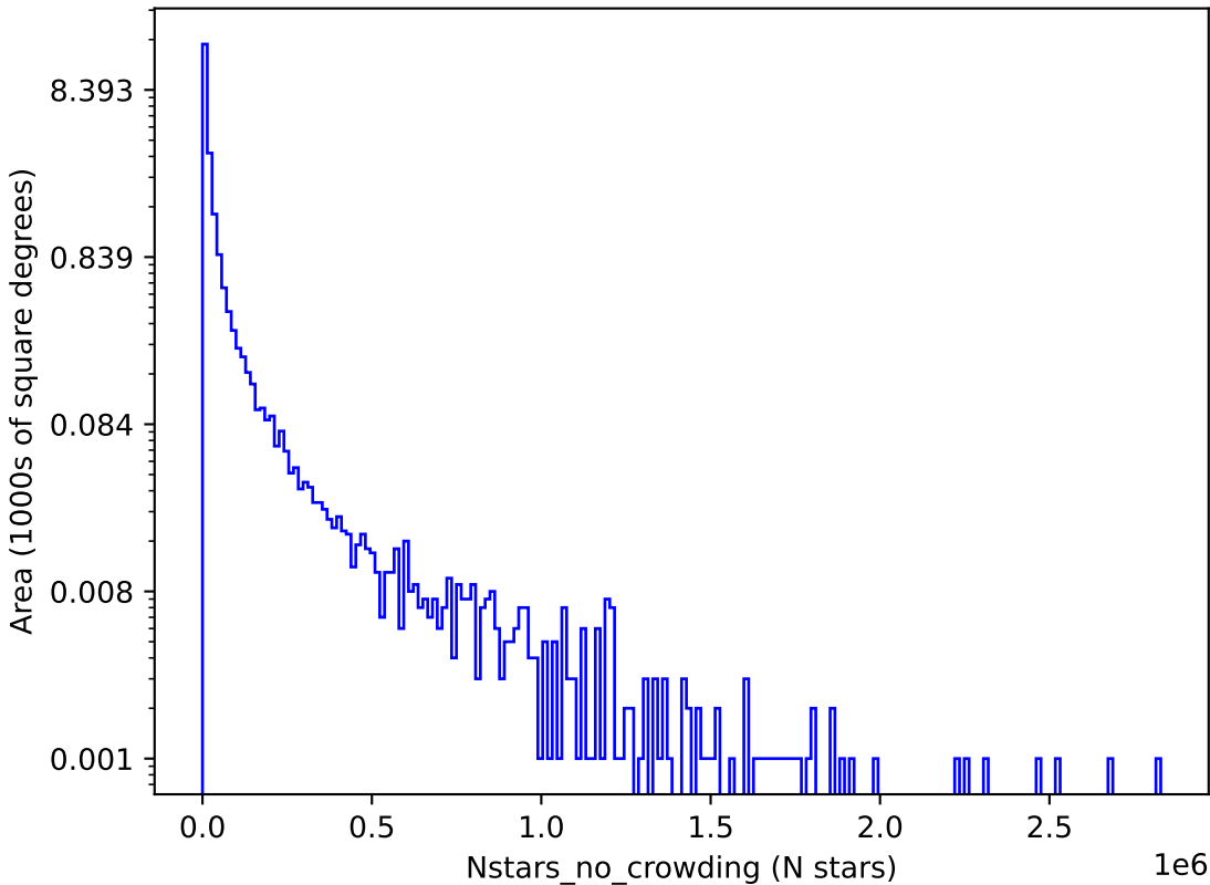
too_elab_r32_d3_gz_v3.4_10yrs u: Nstars_no_crowding
