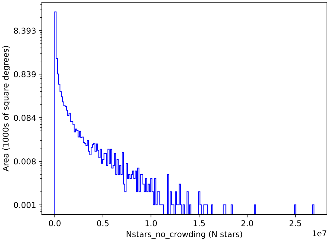
too_elab_r32_d3_gz_v3.4_10yrs i: Nstars_no_crowding
