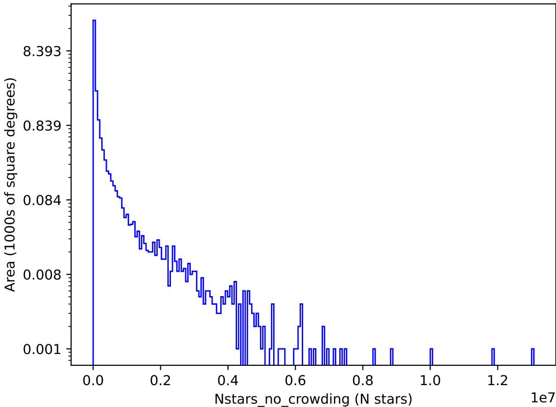
too_elab_r32_d3_gz_v3.4_10yrs g: Nstars_no_crowding
