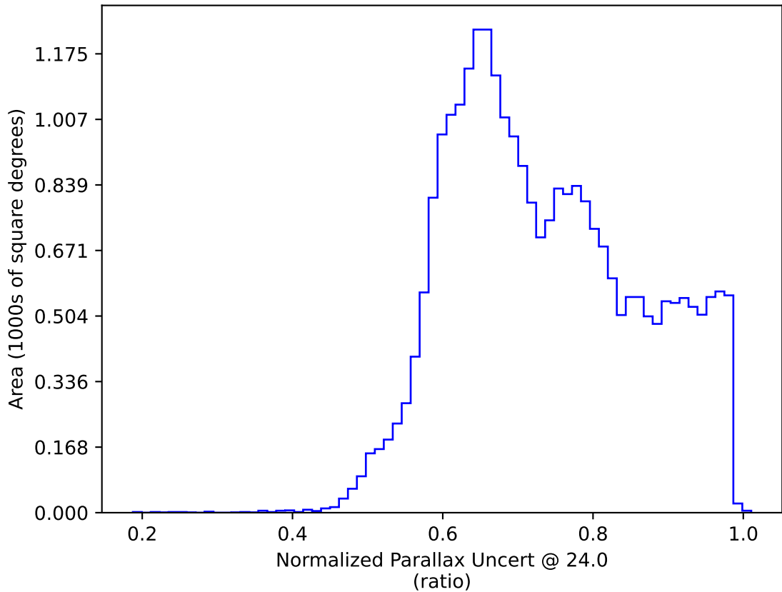
too_elab_r32_d3_gz_v3.4_10yrs : Normalized Parallax Uncert @ 24.0
