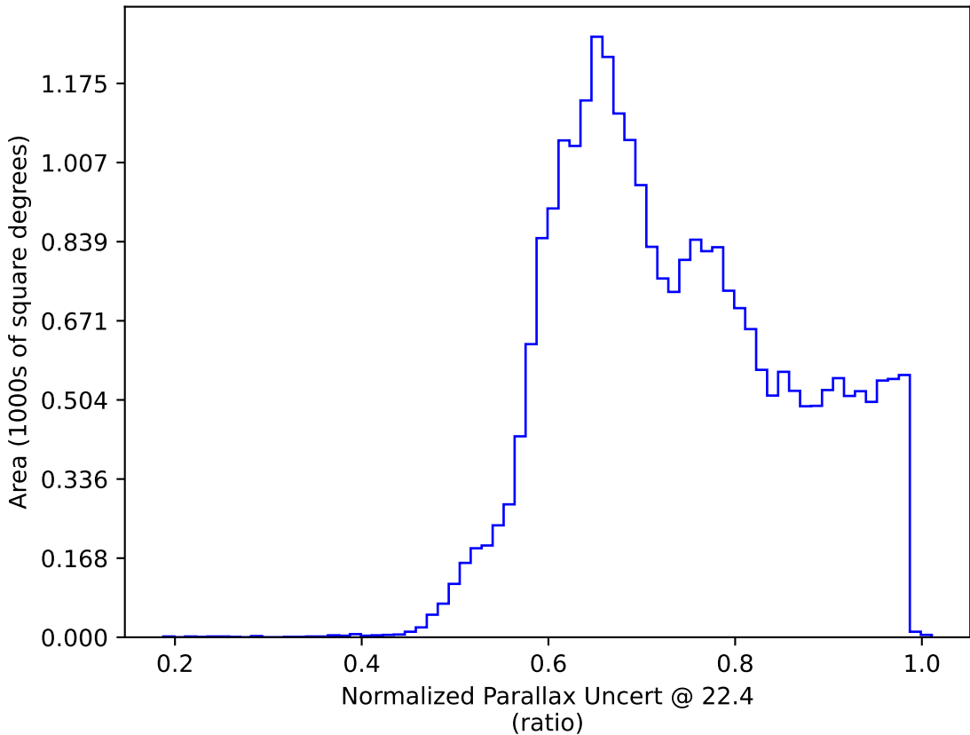
too_elab_r32_d3_gz_v3.4_10yrs : Normalized Parallax Uncert @ 22.4
