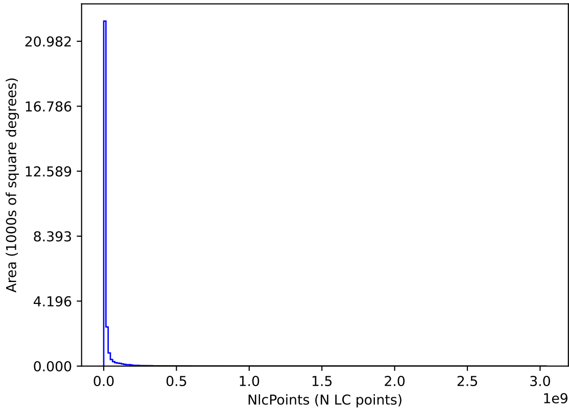
too_elab_r32_d3_gz_v3.4_10yrs : NlcPoints
