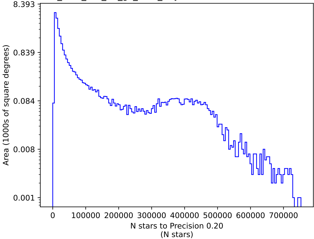
too_elab_r32_d3_gz_v3.4_10yrs i: N stars to Precision 0.20
