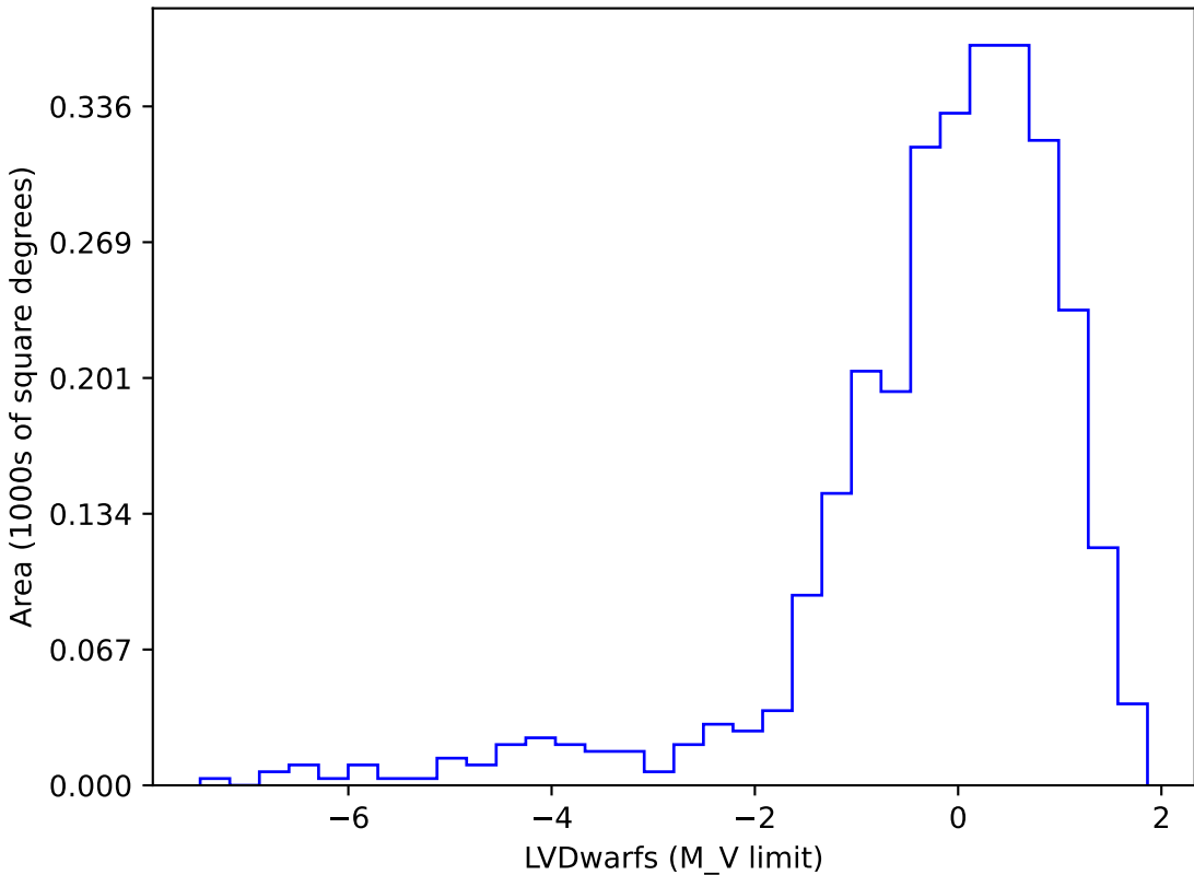
too_elab_r32_d3_gz_v3.4_10yrs gi SCP: LVDwarfs
