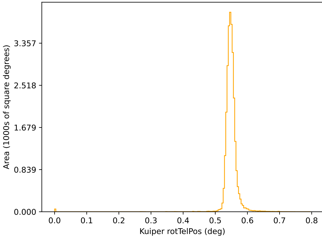
too_elab_r32_d3_gz_v3.4_10yrs r: Kuiper rotTelPos
