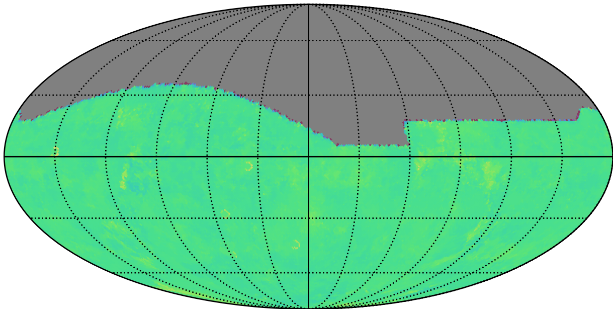
too_elab_r32_d3_gz_v3.4_10yrs g: Kuiper rotTelPos
