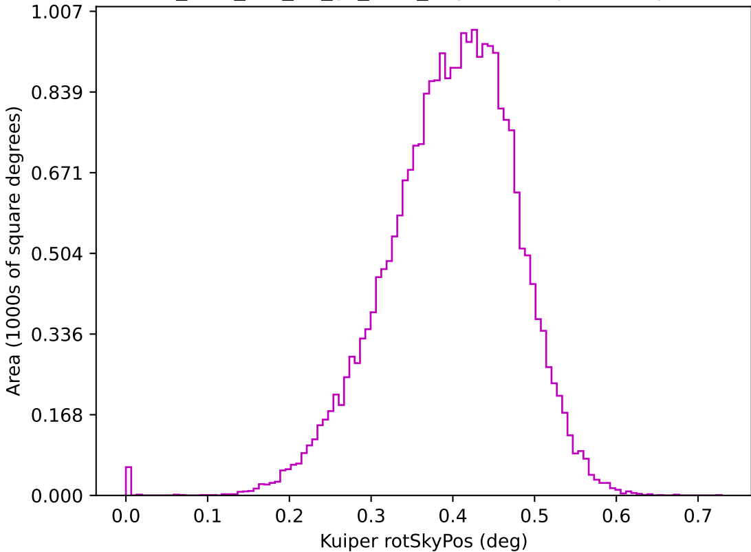
too_elab_r32_d3_gz_v3.4_10yrs z: Kuiper rotSkyPos
