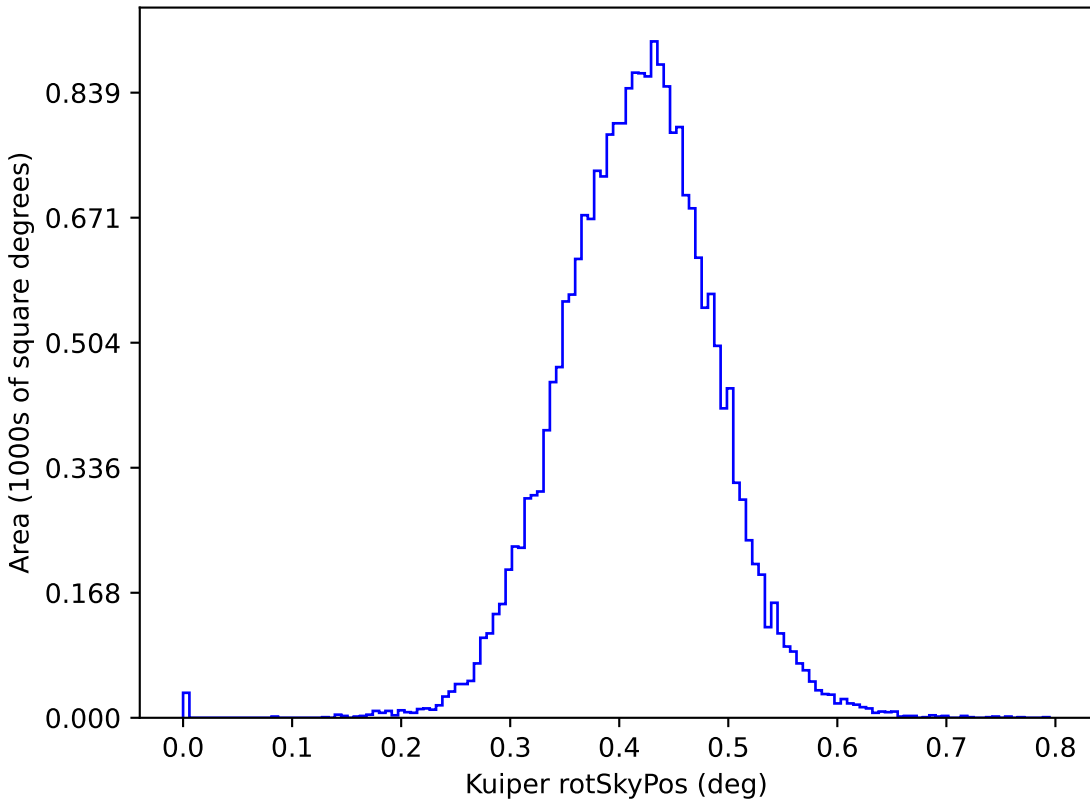
too_elab_r32_d3_gz_v3.4_10yrs y: Kuiper rotSkyPos
