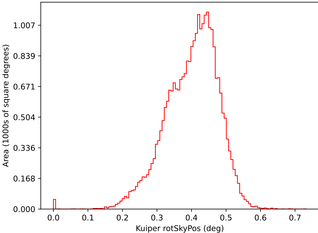
too_elab_r32_d3_gz_v3.4_10yrs i: Kuiper rotSkyPos
