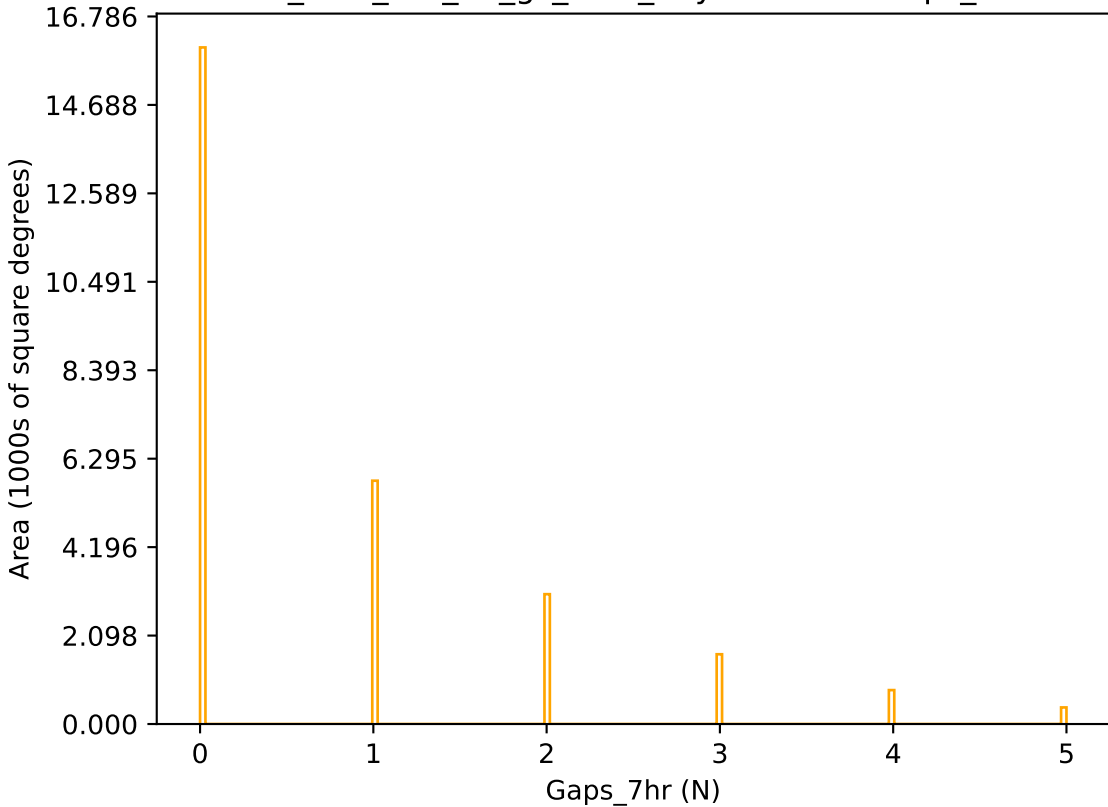
too_elab_r32_d3_gz_v3.4_10yrs r band: Gaps_7hr
