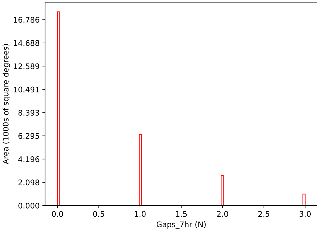
too_elab_r32_d3_gz_v3.4_10yrs i band: Gaps_7hr
