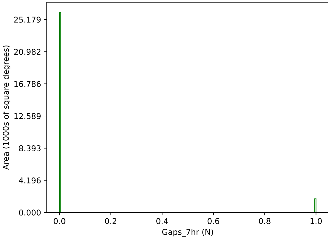
too_elab_r32_d3_gz_v3.4_10yrs g band: Gaps_7hr
