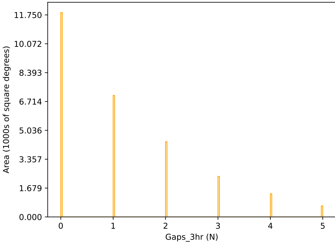
too_elab_r32_d3_gz_v3.4_10yrs r band: Gaps_3hr
