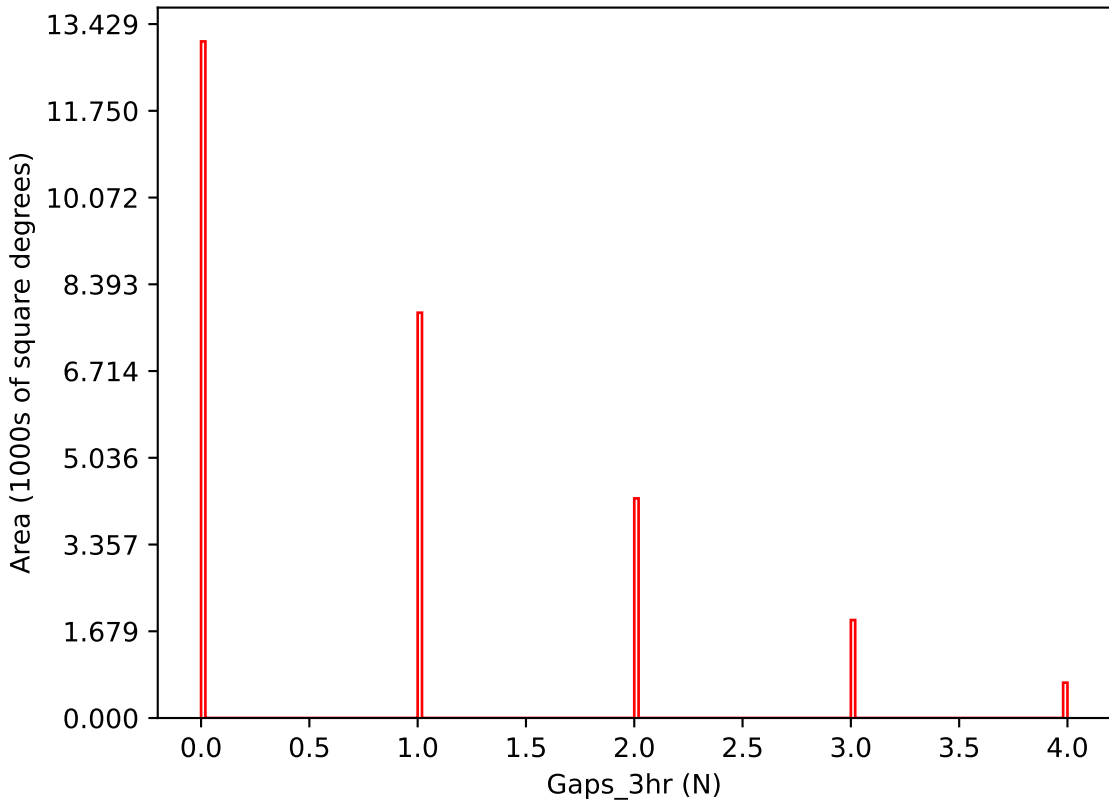
too_elab_r32_d3_gz_v3.4_10yrs i band: Gaps_3hr
