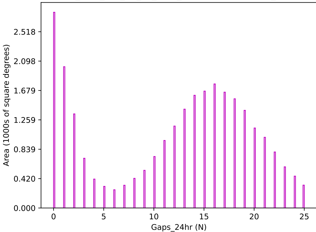
too_elab_r32_d3_gz_v3.4_10yrs z band: Gaps_24hr
