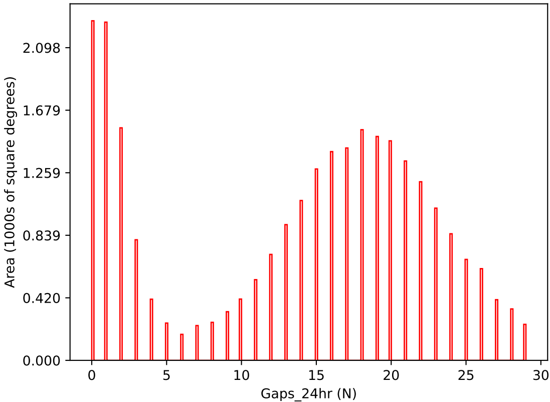
too_elab_r32_d3_gz_v3.4_10yrs i band: Gaps_24hr
