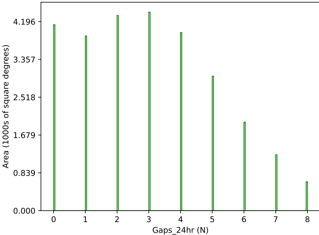
too_elab_r32_d3_gz_v3.4_10yrs g band: Gaps_24hr
