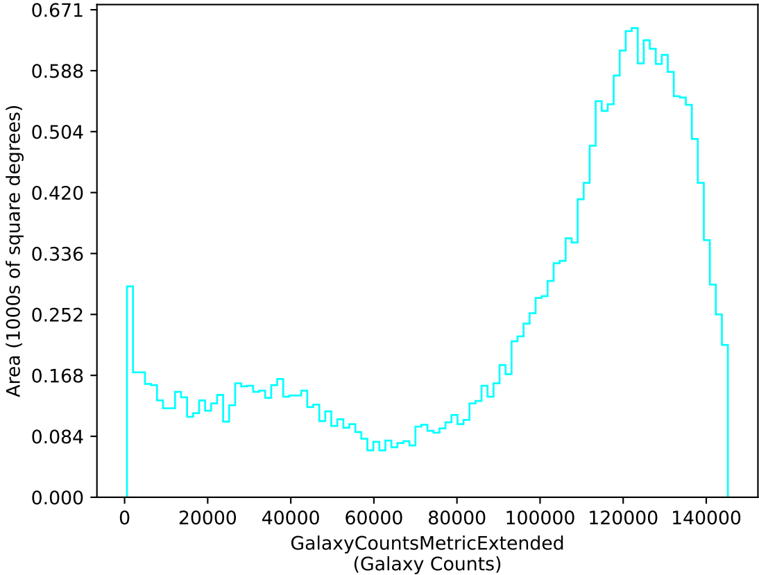
too_elab_r32_d3_gz_v3.4_10yrs u: GalaxyCountsMetricExtended
