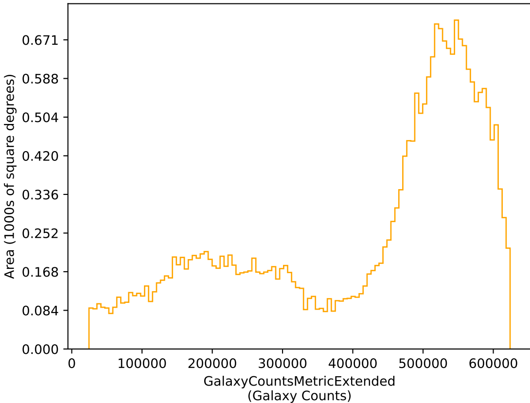
too_elab_r32_d3_gz_v3.4_10yrs r: GalaxyCountsMetricExtended
