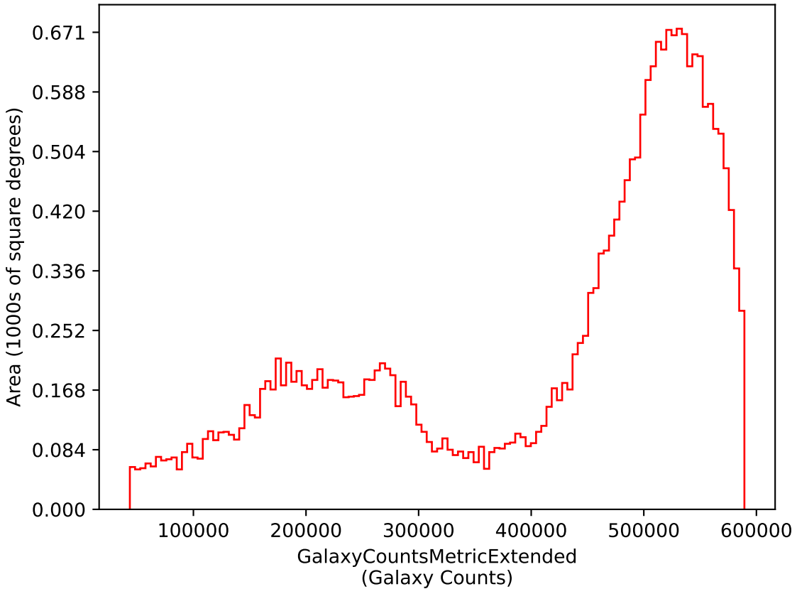
too_elab_r32_d3_gz_v3.4_10yrs i: GalaxyCountsMetricExtended
