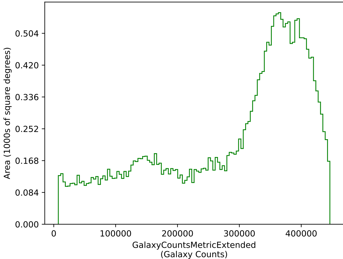
too_elab_r32_d3_gz_v3.4_10yrs g: GalaxyCountsMetricExtended
