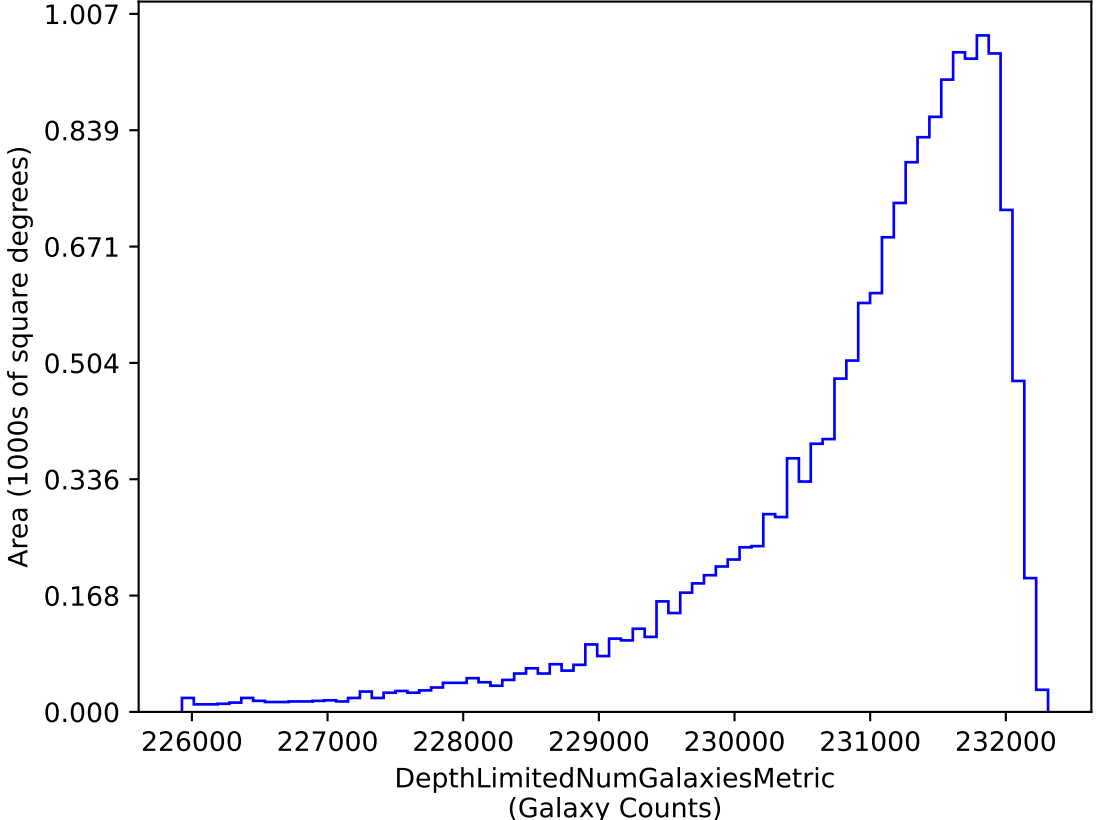
too_elab_r32_d3_gz_v3.4_10yrs i band galaxies non-DD: DepthLimitedNumGalaxiesMetric
