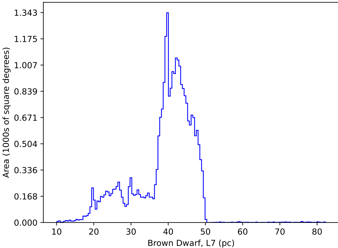
too_elab_r32_d3_gz_v3.4_10yrs : Brown Dwarf, L7
