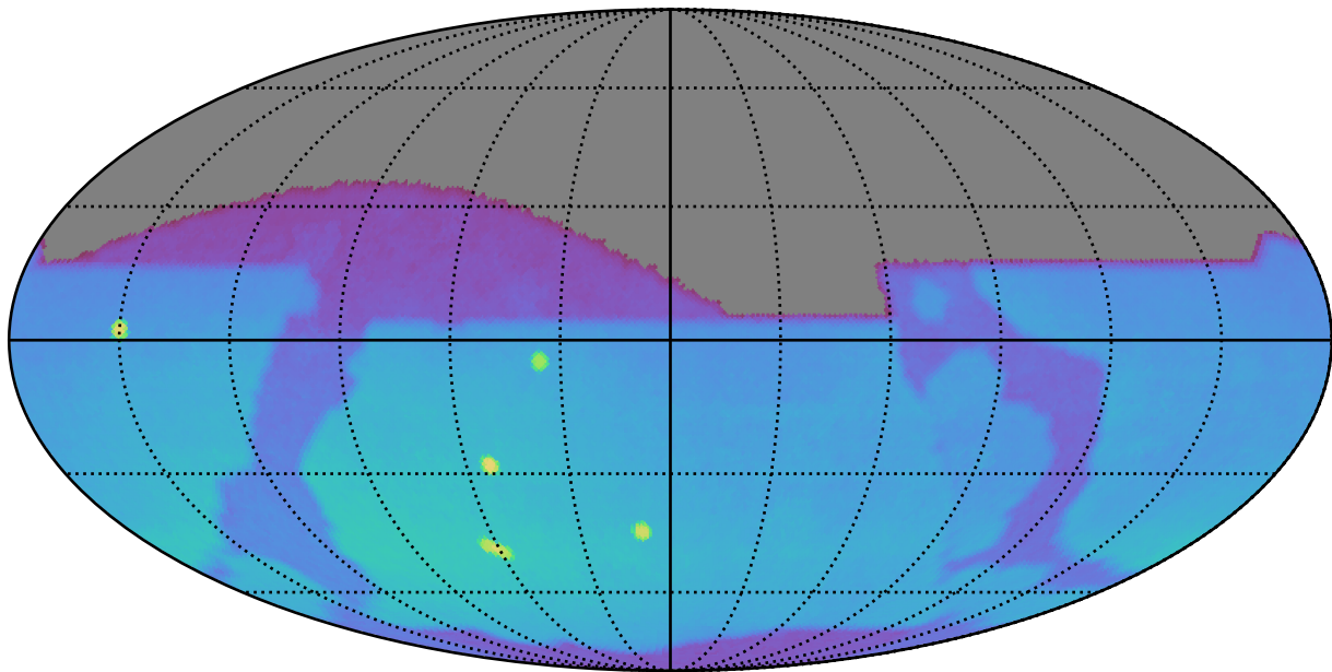
too_elab_r32_d3_gz_v3.4_10yrs : Brown Dwarf, L4
