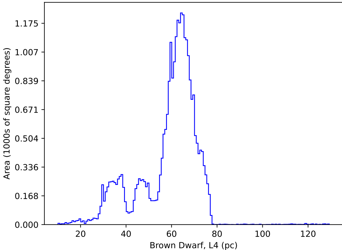
too_elab_r32_d3_gz_v3.4_10yrs : Brown Dwarf, L4
