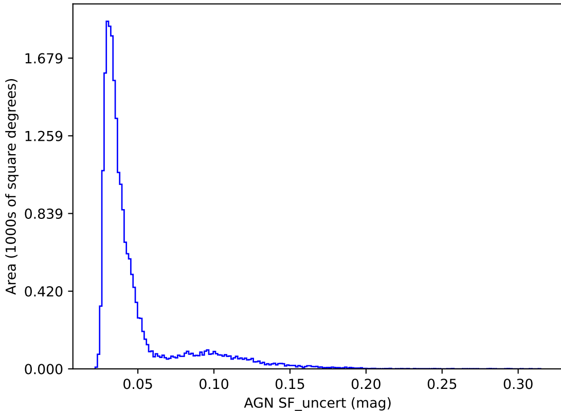
too_elab_r32_d3_gz_v3.4_10yrs y band: AGN SF_uncert
