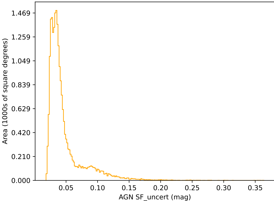
too_elab_r32_d3_gz_v3.4_10yrs r band: AGN SF_uncert
