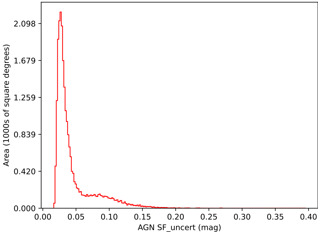
too_elab_r32_d3_gz_v3.4_10yrs i band: AGN SF_uncert
