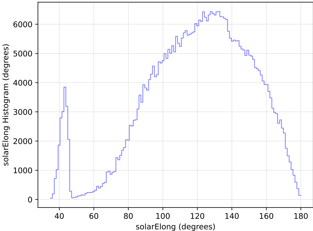
too_elab_r32_d3_gz_v3.4_10yrs WFD z band: solarElong Histogram
