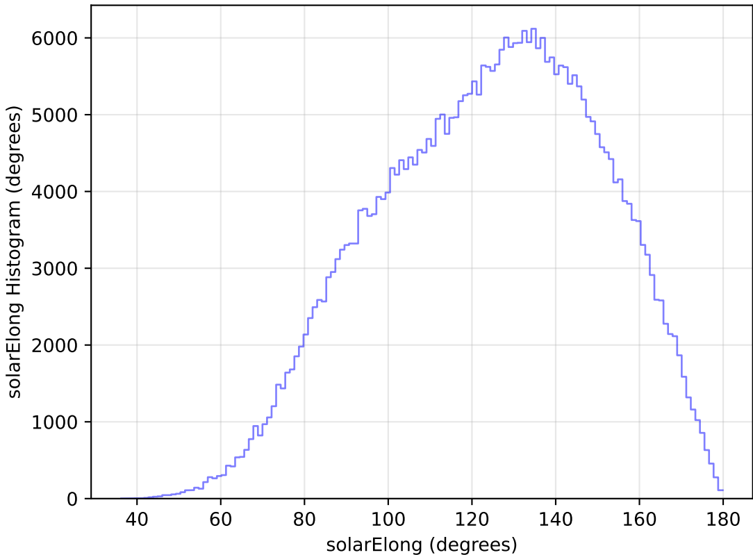
too_elab_r32_d3_gz_v3.4_10yrs WFD y band: solarElong Histogram
