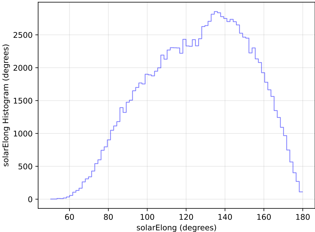
too_elab_r32_d3_gz_v3.4_10yrs WFD u band: solarElong Histogram
