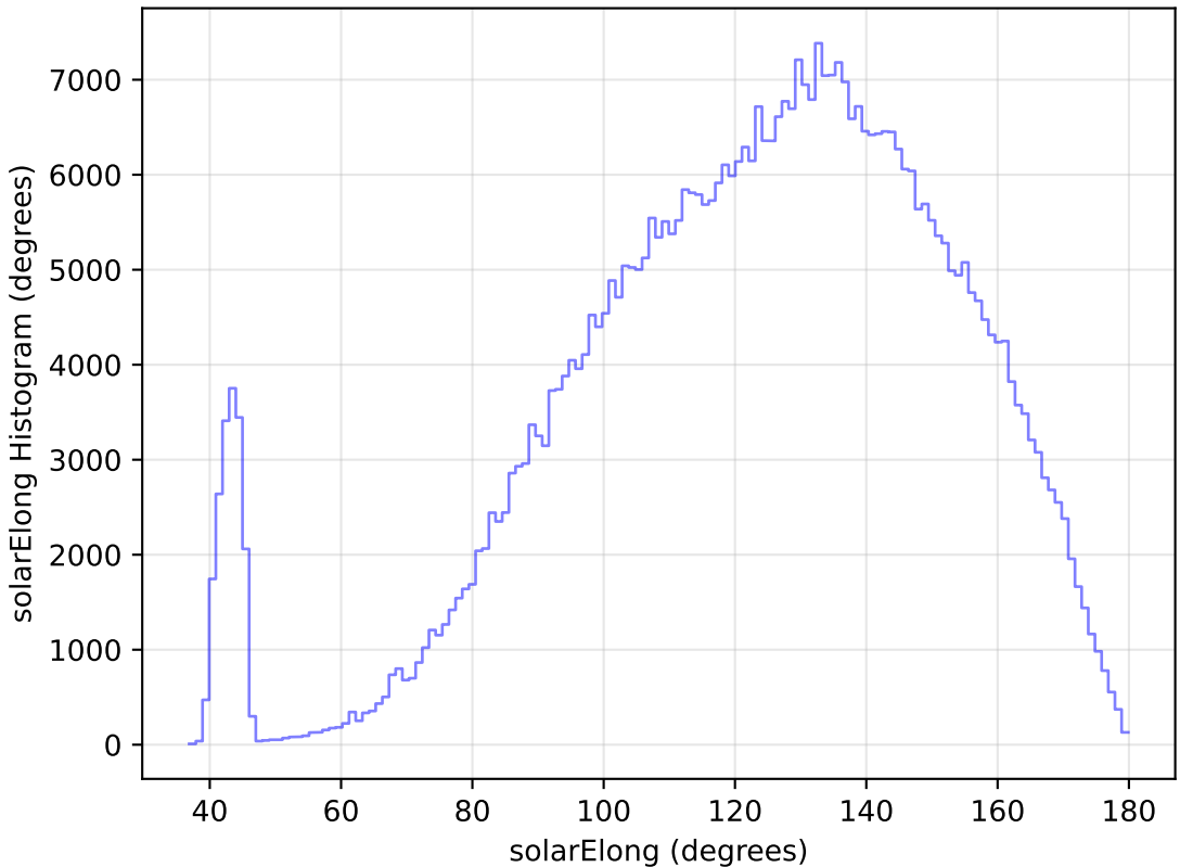
too_elab_r32_d3_gz_v3.4_10yrs WFD r band: solarElong Histogram
