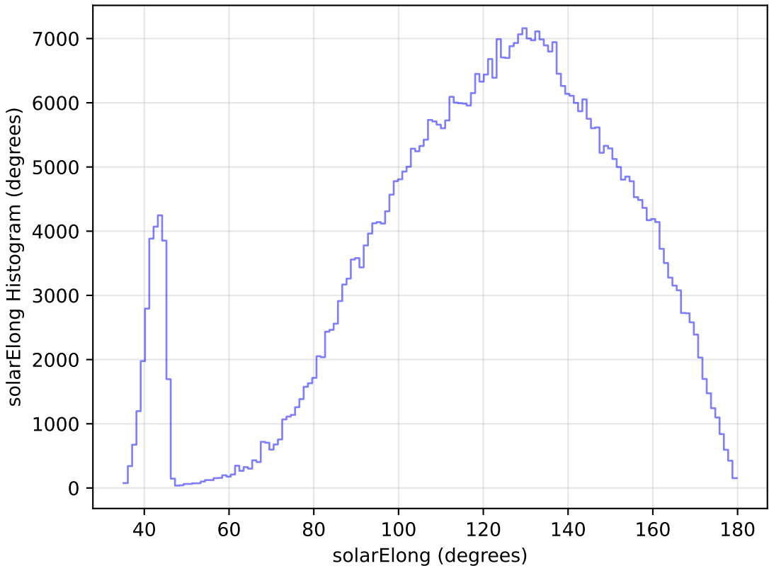
too_elab_r32_d3_gz_v3.4_10yrs WFD i band: solarElong Histogram
