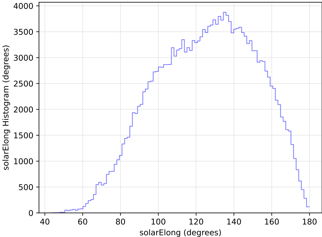
too_elab_r32_d3_gz_v3.4_10yrs WFD g band: solarElong Histogram
