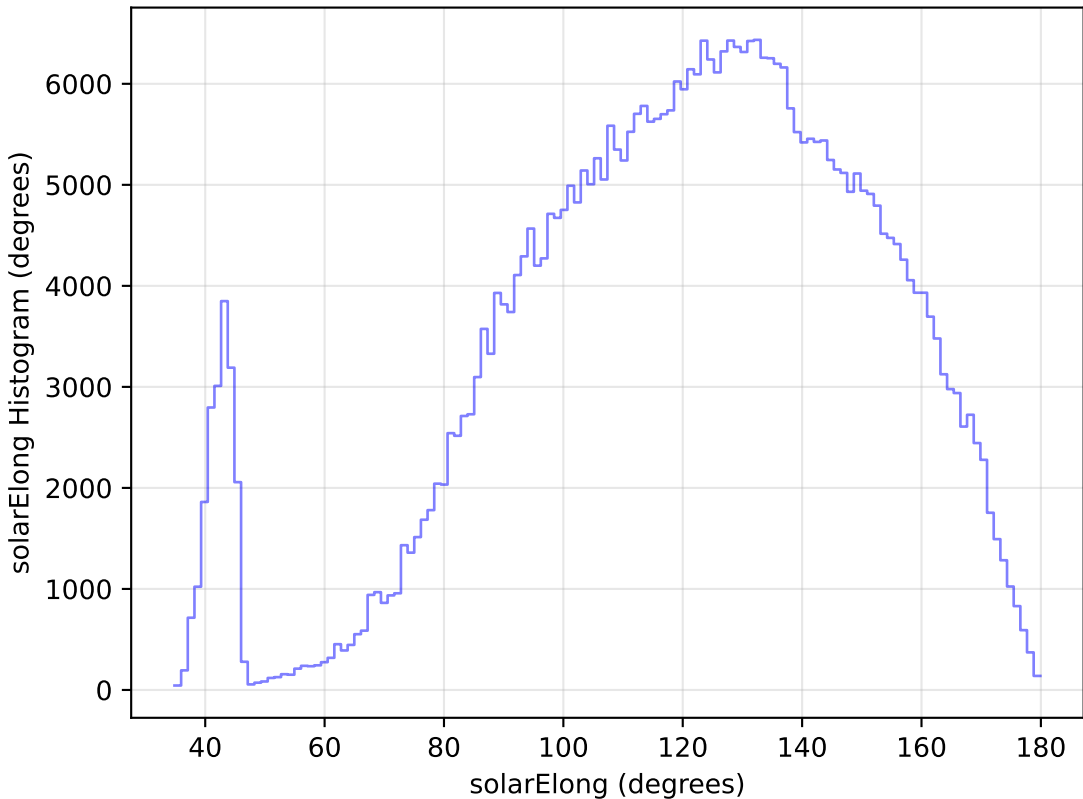
too_elab_r32_d3_gz_v3.4_10yrs All sky z band: solarElong Histogram
