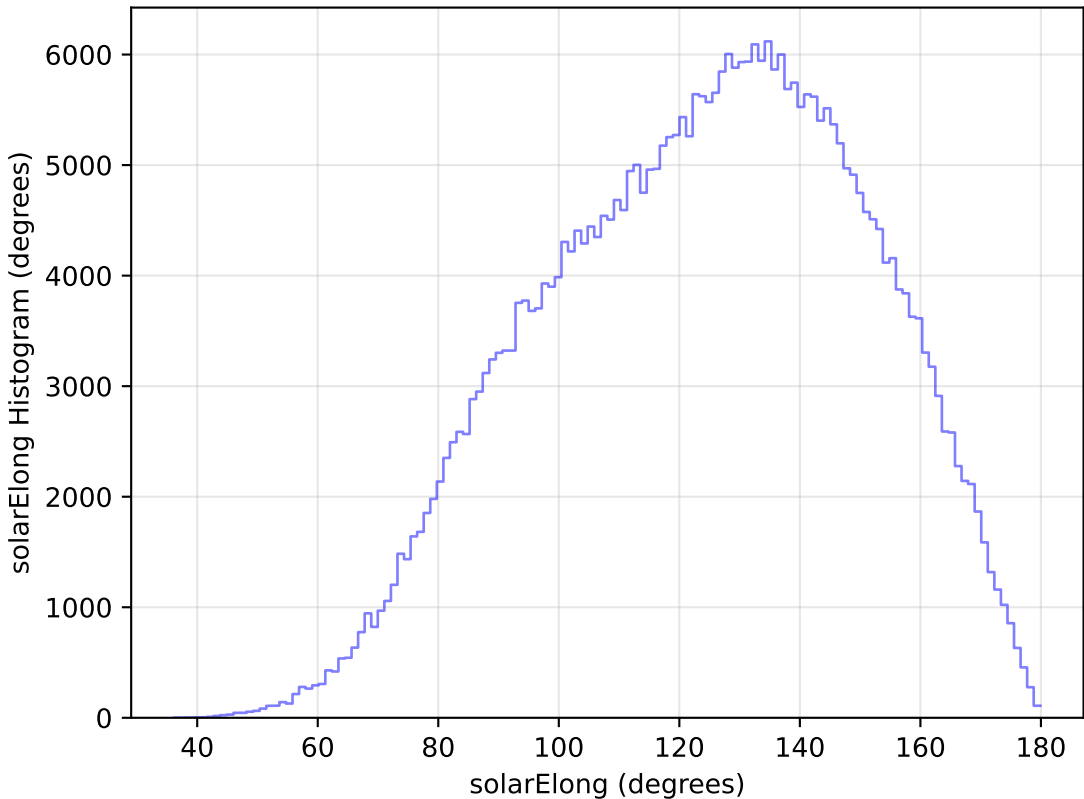
too_elab_r32_d3_gz_v3.4_10yrs All sky y band: solarElong Histogram
