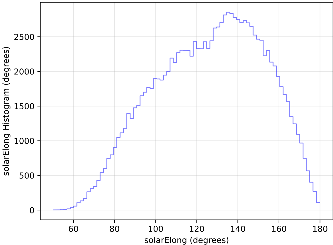
too_elab_r32_d3_gz_v3.4_10yrs All sky u band: solarElong Histogram
