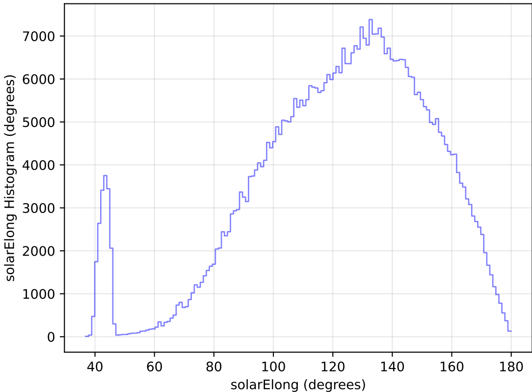
too_elab_r32_d3_gz_v3.4_10yrs All sky r band: solarElong Histogram
