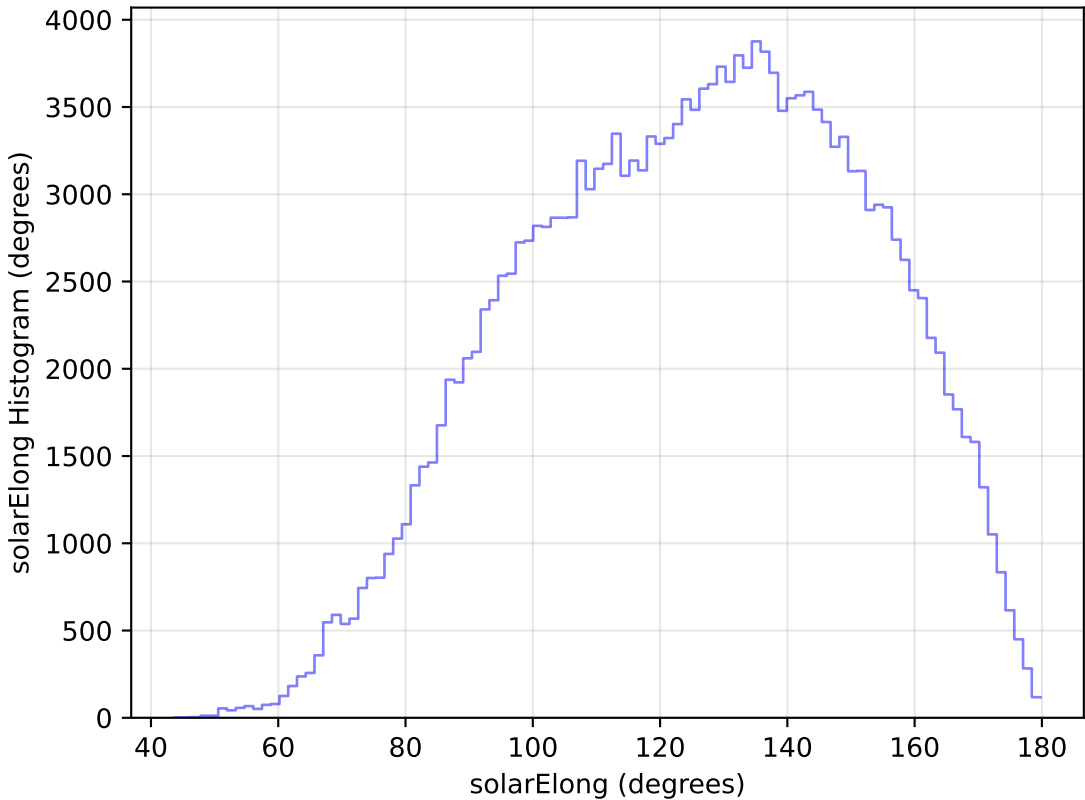
too_elab_r32_d3_gz_v3.4_10yrs All sky g band: solarElong Histogram
