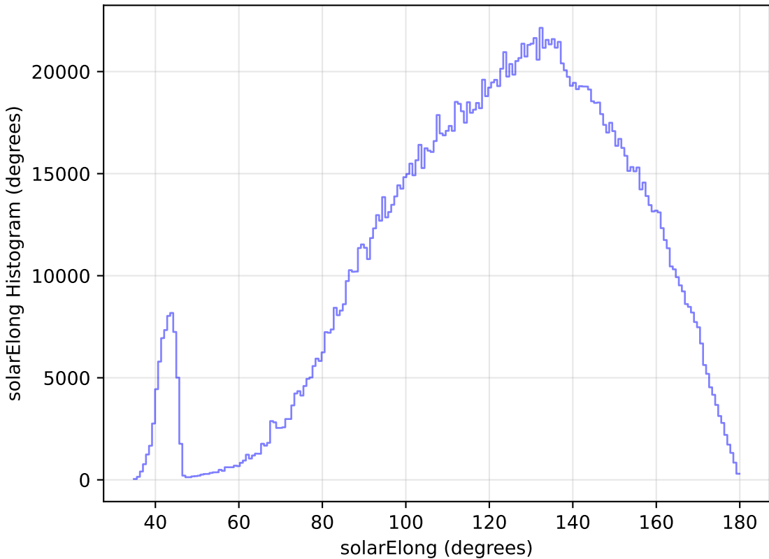
too_elab_r32_d3_gz_v3.4_10yrs All sky all bands: solarElong Histogram
