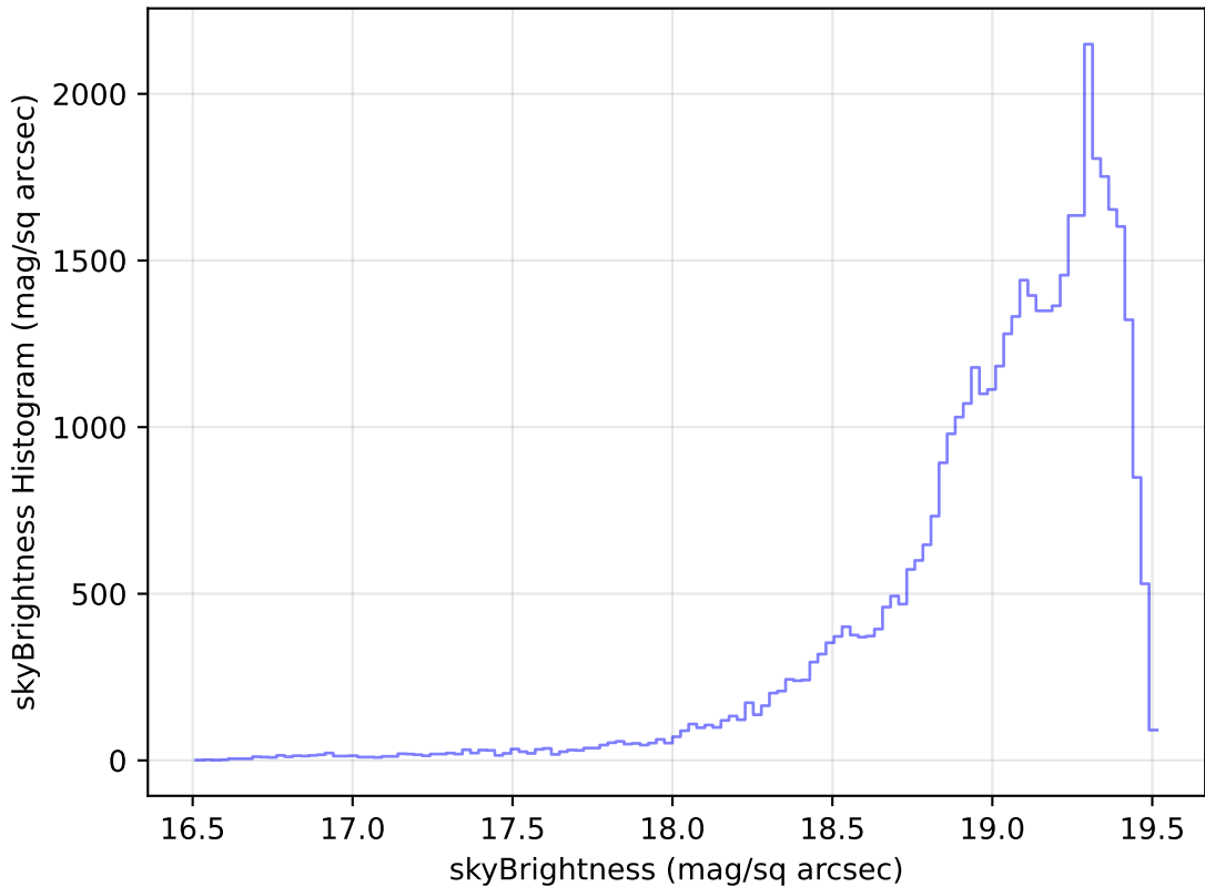
too_elab_r32_d3_gz_v3.4_10yrs Yr 1 z band: skyBrightness Histogram
