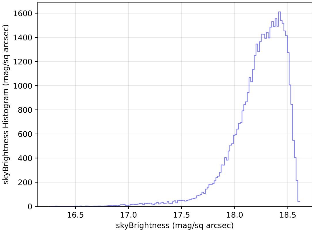
too_elab_r32_d3_gz_v3.4_10yrs Yr 1 y band: skyBrightness Histogram
