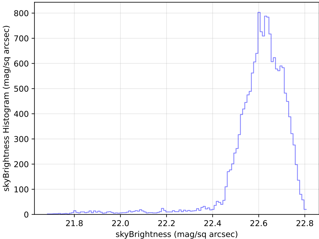
too_elab_r32_d3_gz_v3.4_10yrs Yr 1 u band: skyBrightness Histogram
