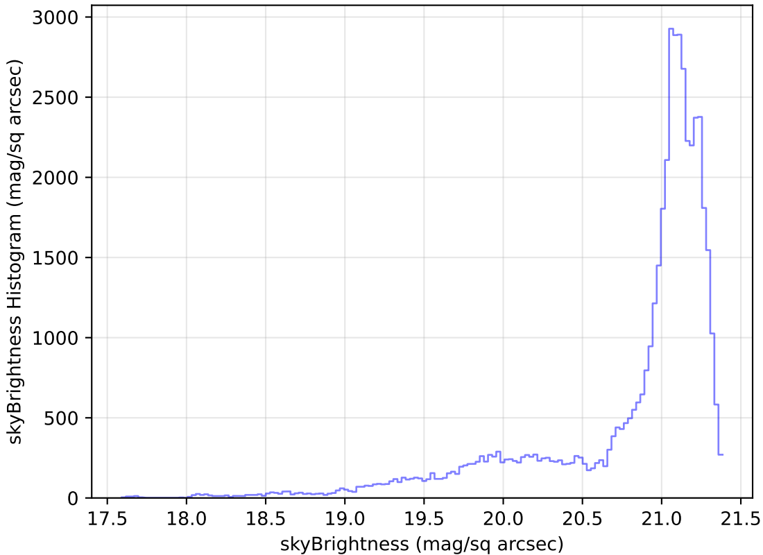
too_elab_r32_d3_gz_v3.4_10yrs Yr 1 r band: skyBrightness Histogram
